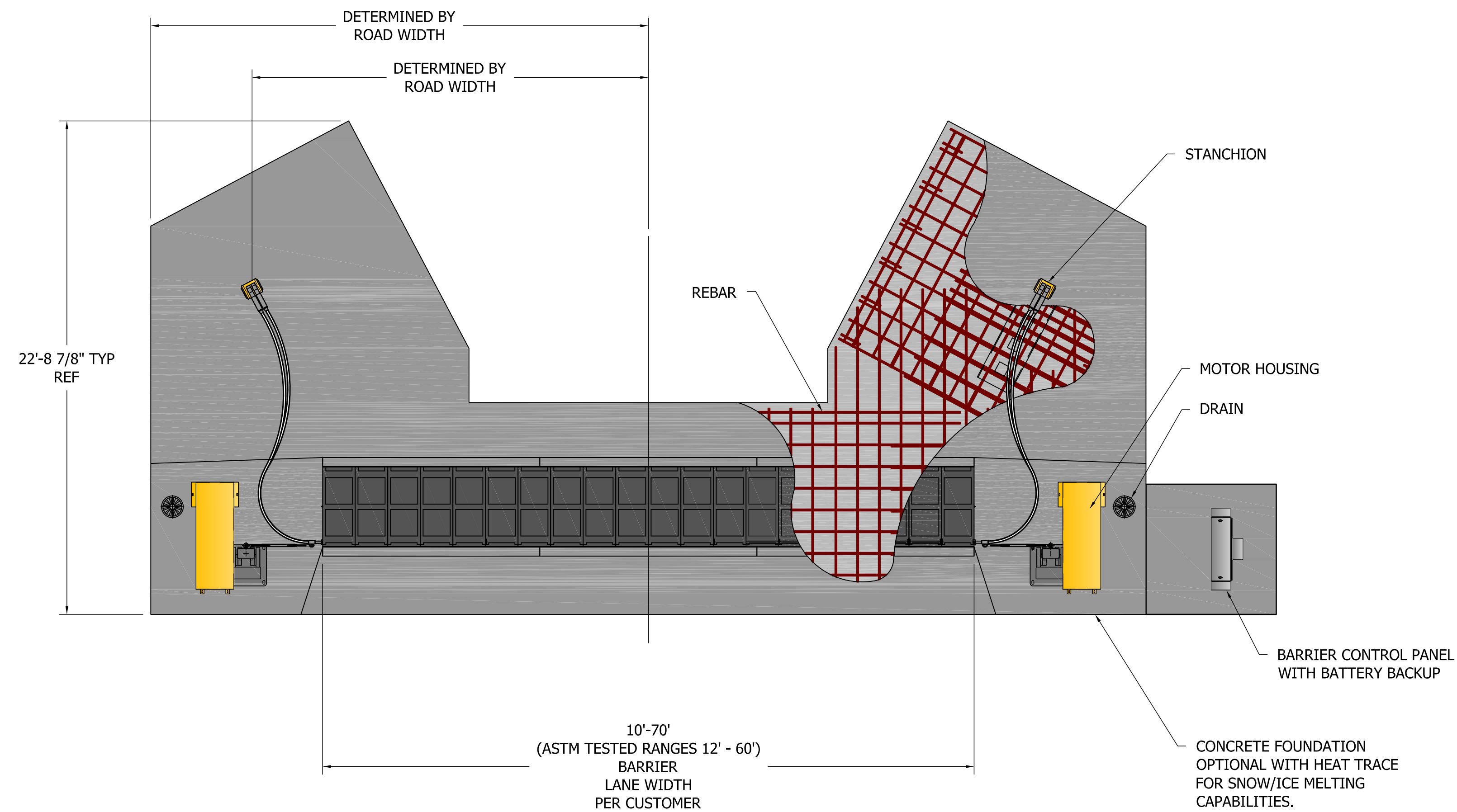
A - PLAN VIEW SCALE: 1/4" = 1'-0"
