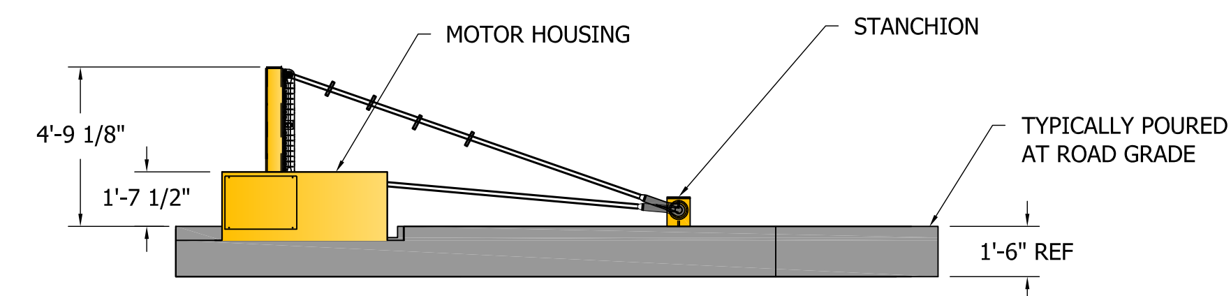
A-2 - SIDE ELEVATION VIEW SCALE: 1/4" = 1'-0"
